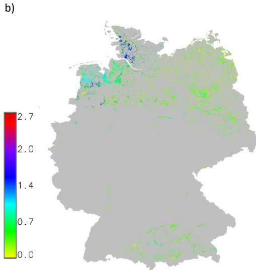
Fig.: Regionalized GHG emissions of organic soils a) \text{CO}_2 [ \text{g CO}_2 \text{ C m}^{-2} \text{ a}^{-1} ]; b) \text{N}_2\text{O} [ \text{N}_2\text{O N ha}^{-2} \text{ a} ]
